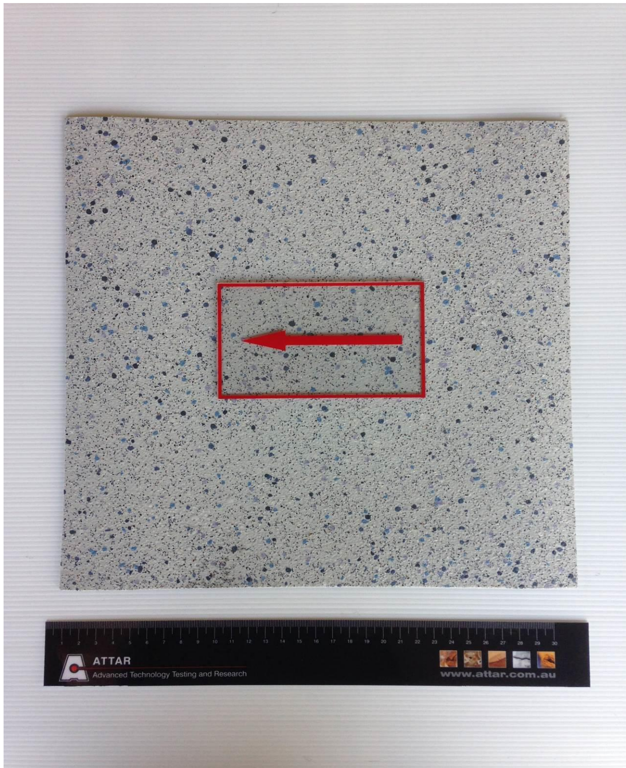
Figure 1: Safetred Spec – Highlighted area indicates area tested and direction of test.
