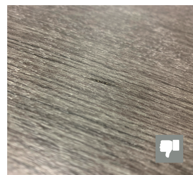
results NOK after 25000 cycles; the wear layer has been damaged
