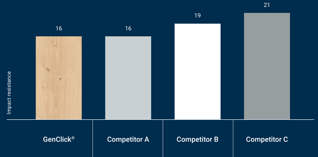
GRAPH 2: IMPACT RESISTANCE (INTERNAL TEST) LOWEST SCORE = HIGHEST RESISTANCE TO IMPACT
