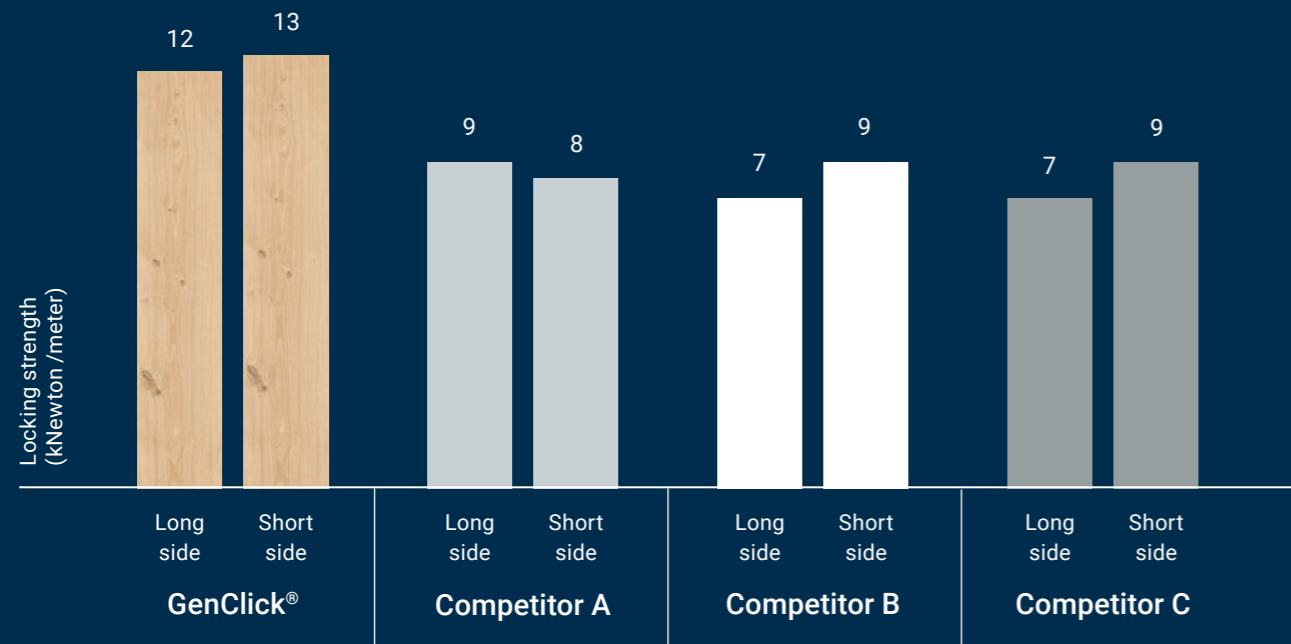
GRAPH 1: LOCKING STRENGTH (ISO 10582) HIGHER LOCKING STRENGTH SCORE = STRONGER CONNECTION
