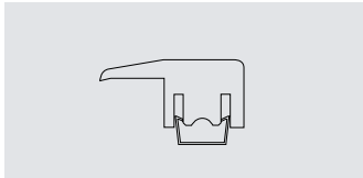
End profile DIMENSIONS (LxWxH): 2000x38x19 mm FLOOR THICKNESS: 13-17 mm OAK: 8791136 OAK, UNFINISHED: 8791134
