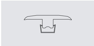
Transition profile DIMENSIONS (LxWxH): 2000x44x12 mm FLOOR THICKNESS: 8-12 mm OAK: 8791175
