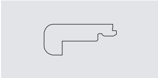
Stair nosing DIMENSIONS (LxWxH): 2000x60x26 mm FLOOR THICKNESS: 14 mm, 2-lock OAK: 8791466 OAK, UNFINISHED: 8791465
