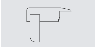
Stair nosing / landing profile DIMENSIONS (LxWxH): 2000x66x20/40x14 mm FLOOR THICKNESS: 13-14 mm OAK: 8791446
