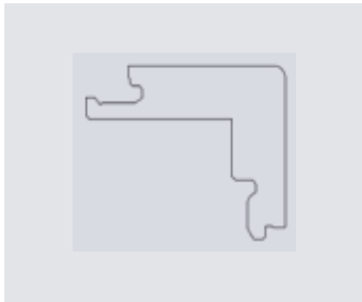
Stair nosing - Integrated 2 Used to make a fully integrated solution for closed steps. To be glued down. DIMENSIONS (LxWxHxT): 1950x52x44x14 FLOOR THICKNESS: 14 mm, 2-lock OAK, UNFINISHED: 8795042
