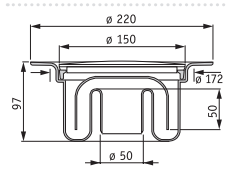
SIPHON PURUS DUSCH BRUNN 50 ref. 1416 001 outflow 2L/s
