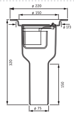
SIPHON STAINLESS STEEL 40* ref. 1416 007 outflow 0.25L/s
