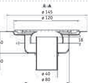
SIPHON STAINLESS STEEL 40* ref. 1416 007 outflow 0.25L/s
