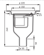
SIPHON PURUS DUSCH BRUNN 50 ref. 1416 001 outflow 2L/s
